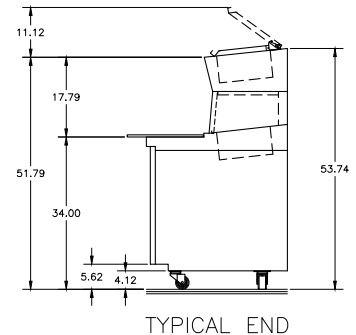
TYPICAL END
