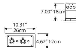
N8744-R Remote Control Cutout Dimensions
